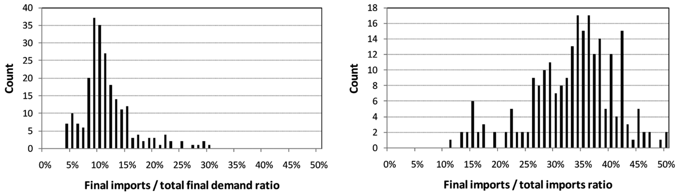
Figure 3. (a) Frequency count of the final imports/total final demand ratio; (b) frequency count of the final imports/total imports ratio. Compiled based on national input-output tables of Argentina, Australia, Austria, Belgium, Brazil, Canada, Chile, China, Czech Republic, Germany, Denmark, Spain, Estonia, Finland, France, UK, Greece, Hong Kong, Hungary, Indonesia, India, Ireland, Israel, Italy, Japan, Korea, Lithuania, Latvia, Mexico, Macedonia, Malaysia, Netherlands, Norway, New Zealand, Philippines, Poland, Portugal, Romania, Russia, Singapore, Slovakia, Slovenia, Sweden, Thailand, Turkey, Taiwan, United States, and South Africa, dated between 1990 and 2007.
