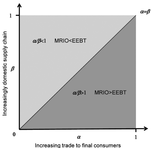
Figure 4. Schematic illustrating the differences between emissions embodied in trade determined by the MRIO and EEBT methods.
