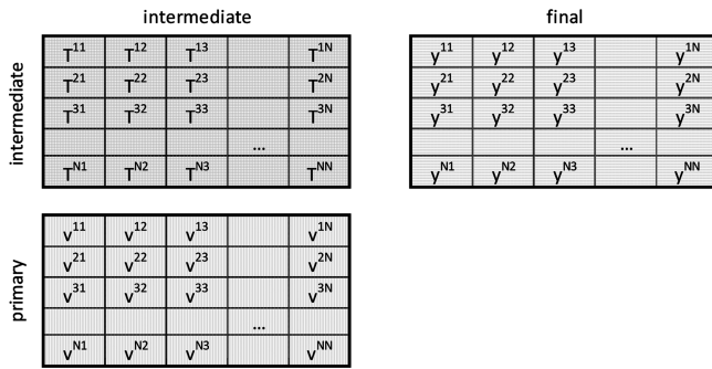
Figure 1. Global accounting balance in an MRIO. Vertically hatched: sums of sectoral inputs, must equal horizontally hatched: sums of sectoral outputs. Note that block descriptors are given with sector indices, for example, T^{32} is a matrix with elements T_{ij}^{32} . Note also that the entire intermediate demand block T including intermediate trade T_{ji}^{sr} \neq s cancels out (see eq 2).
