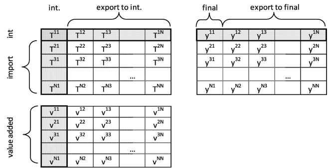
Figure 2. National Accounting Balance in an MRIO (exemplary for region 1). Vertically hatched: sums of sectoral inputs, must equal horizontally hatched: sums of sectoral outputs. Note that only the intraregion intermediate (int) demand block T^{11} cancels out (see eq 3). In MRIO exports are separated into exports to intermediate (int) and final consumption (as shown).
