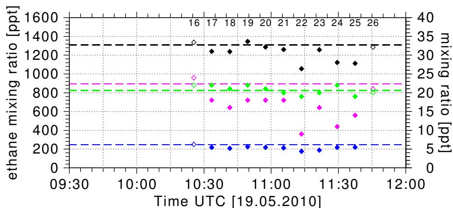
Fig. 9. Selected non-methane hydrocarbons (NMHCs) and perchloroethylene (PCE) measurements in whole air samples collected on 19 May 2010. Same representation as in Fig. 6.
