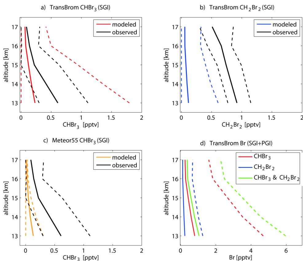
Fig. 5. VLS profiles based on atmospheric observations (black lines) and estimated from observed emissions (colored lines) of West Pacific \text{CHBr}_3 (a), West Pacific \text{CH}_2\text{Br}_2 (b), and tropical Atlantic \text{CHBr}_3 (c) are shown. Also total Br profiles (PG and SG) based on West Pacific \text{CHBr}_3 and \text{CH}_2\text{Br}_2 emissions are displayed (d). For all profiles lower and upper limits (dashed lines) and mean values (solid lines) are given.
