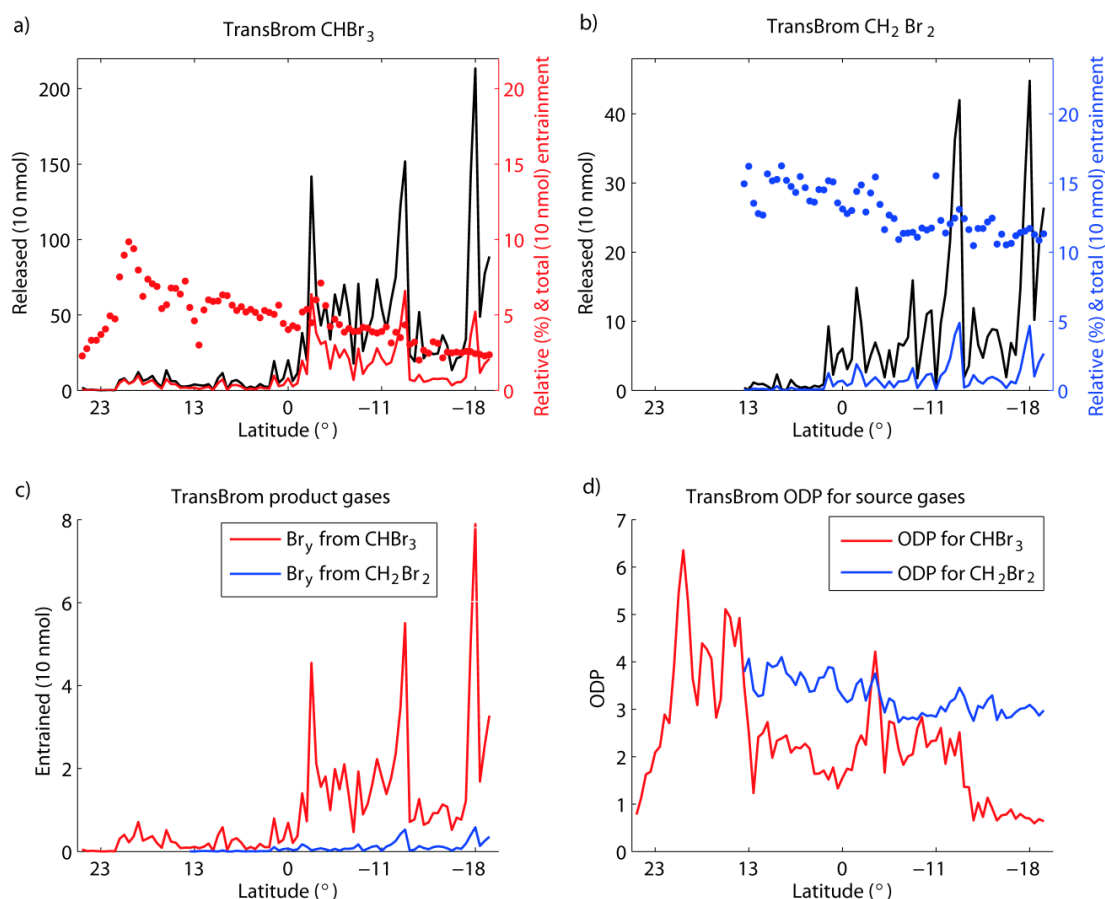
Fig. 3. Observed emissions of VSLs for one hour over 500 m 2 (black line), and relative (colored dots) and total (colored line) amount of VSLs entrained above 17 km for CHBr 3 (a) and CH 2 Br 2 (b) are shown. PGI is given based on CHBr 3 and CH 2 Br 2 emissions (c). Ozone depletion potential as a function of emission location is displayed for both VSLs (d).
