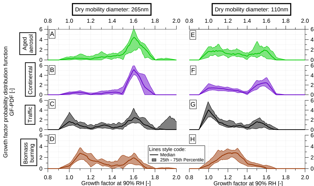
Fig. 13. Median (thicker lines) as well as 25 th and 75 th percentiles (thin lines and shading) of GF-PDF at RH = 90 %, for each air mass type/aerosol source and for two dry particle mobility diameters: 265 nm (left panels) and 110 nm (right panels).
