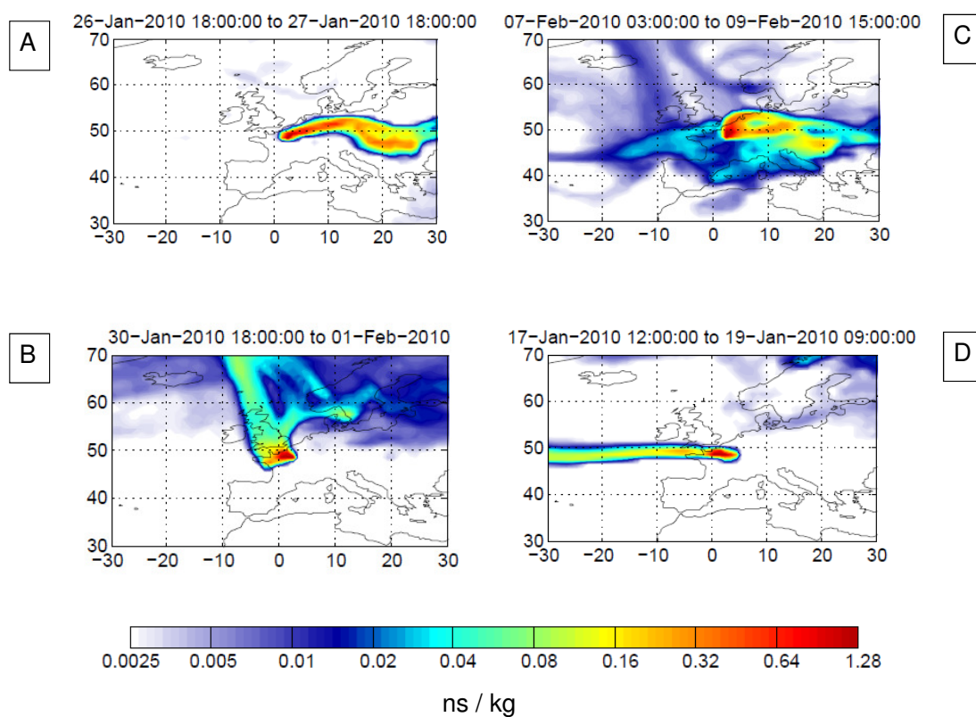
Fig. 5. Typical footprint potential emission sensitivities, from FLEXPART retroplume calculations. The X-axis represents the longitude while the Y-axis represents the latitude. Calculations are made for (A) and (C) the continental influence, (B) the biomass burning influence (SP2 coupled to HTDMA in this case), (D) the aged aerosol influenced air mass.
