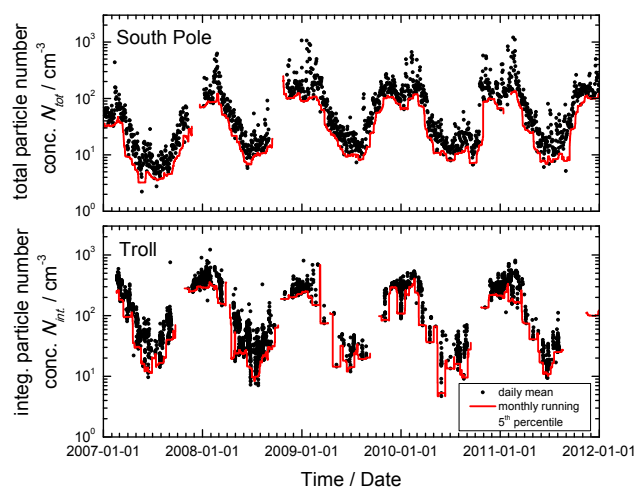
Fig. 3. Time series (2007–2011) of daily averaged total particle number concentration N_{tot} measured by condensation particle counter (CPC) at South Pole station (top panel, black dots), and corresponding time series of particle number concentration integrated over the PNSD N_{int} measured by DMPS at Troll station (bottom panel, black dots). To highlight the annual cycle also in the particle number concentration, the plots contain the respective running 4-week 5th percentiles (red lines), which are again based on hourly values.
