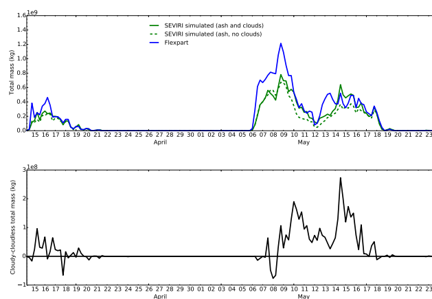
Figure 11. Ash retrieval time series for the Eyjafjallajökull (2010) eruption: total ash cloud mass from the Flexpart model (blue line) and as retrieved from simulated cloudless (green dashed line) and cloudy (green solid line) SEVIRI scenes (top). The difference between the cloudy and cloudless simulation from the above plot (bottom). Note that only coincident pixels are included in both plots.
