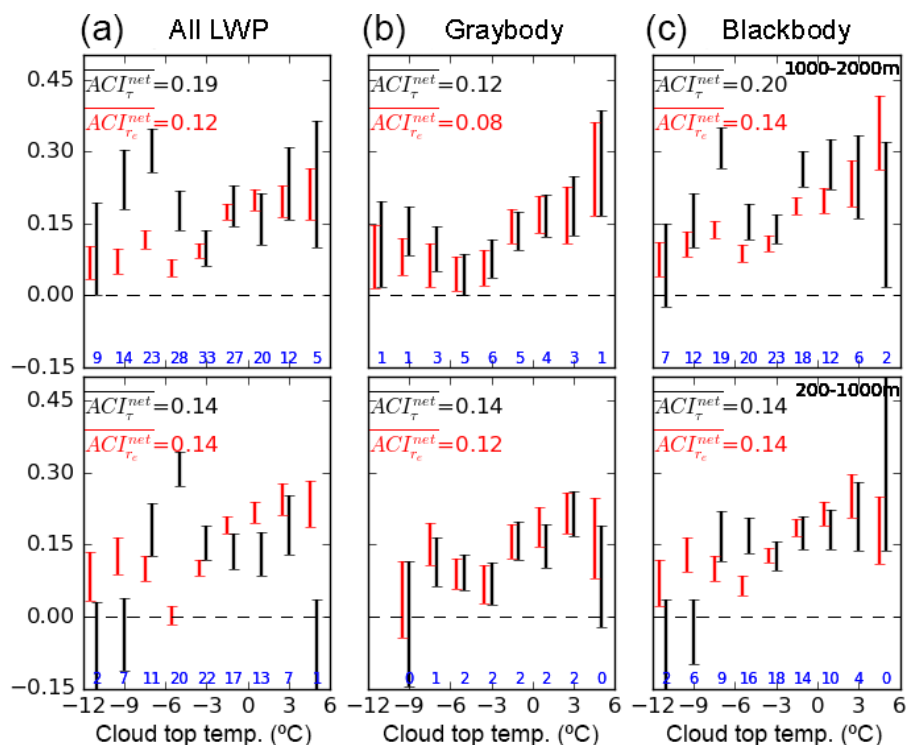
Figure 5. ACI^{\text{net}} parameter of the effective radius ( r_e ) (red) and optical depth ( \tau ) (black), as a function of temperature calculated for liquid clouds between 200–1000 m (lower row) and 1000–2000 m (upper row). The bars indicate the 95 % confidence limit in the calculation of the mean ACI^{\text{net}} value. Each column corresponds to different thresholds for LWP (blackbody: LWP > 40 \text{ g m}^{-2} , graybody: LWP < 40 \text{ g m}^{-2} ). Blue numbers indicate the number of grid cells, in hundreds, that are used to calculate each ACI^{\text{net}} value. In each figure the ACI^{\text{net}} value averaged over the temperature and weighted according to the inverse of the uncertainty is indicated.
