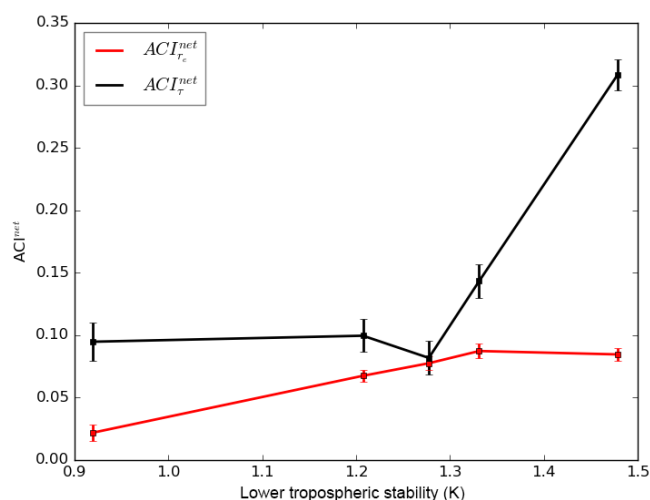
Figure 7. ACI_{r_e}^{net} (red) and ACI_{\tau}^{net} (black) and ACI_{\tau}^{net} as a function of the lower tropospheric stability, stratified by specific humidity between 2.0 and 4.0 \text{g kg}^{-1} .
