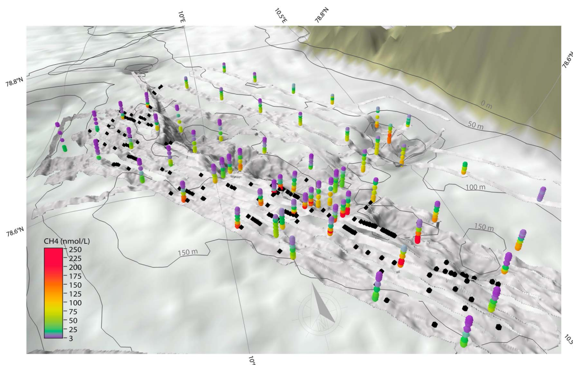
Figure 3. \text{CH}_4 concentrations from a hydrocast survey offshore of Prins Karls Forland. The first three bottles were taken 5, 15, and 30 m above the seafloor, and the last three bottles were taken 10, 20, and 30 m below the sea surface. The rest of the samples were spread equally in the water column depending on the bottom depth. \text{CH}_4 concentrations in the ocean are illustrated by colored dots (scale on the bottom left in \text{nmol L}^{-1} ). Black dots indicate the location of the gas flares. Isobaths are from International Bathymetric Chart of the Arctic Ocean version 3 grid and the superimposed higher resolution bathymetry is from the multibeam survey performed during the R/V Helmer Hanssen cruise; data were recorded over the period 25 June to 1 July 2014.
