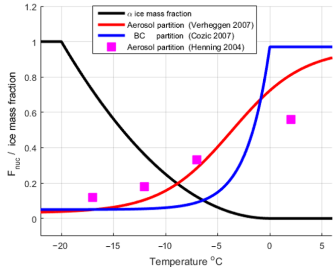
Figure 1. The fraction of cloud water that is in the ice phase ( \alpha ) if CTWC is used (black line) and the fraction of aerosols that reside within cloud droplets ( F_{nuc} ) (colored lines and dots) as a function of temperature. For F_{nuc} , partitioning values for aerosol number from Verheggen et al. (2007) (red line), from Henning et al. (2004) (magenta dots) and from Cozic et al. (2007) (valid for black carbon (BC) particles) are shown. For the BC partitioning, ice fraction was converted to temperature using \alpha .
