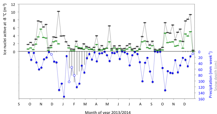
Figure 2. Time course of INP -8 in the PM 10 (black) and PM 2.5 (green) particle size fractions. Peaks in INP -8 largely mirror peaks in precipitation (blue is inverse scale to mirror precipitation values on the horizontal axis). Snow (open circles) or small amounts of rain are accompanied by very small numbers of INP -8 in the same week. Significant amounts of snow on the ground (grey bars) seem to attenuate the increase in INP -8 with intense rainfall. Total amount of precipitation in 2014 was 2077 mm (entire period shown: 2640 mm). Precipitation and snow cover data are the averages of three stations operated by the Norwegian Meteorological Institute in the municipality of Birkenes.
