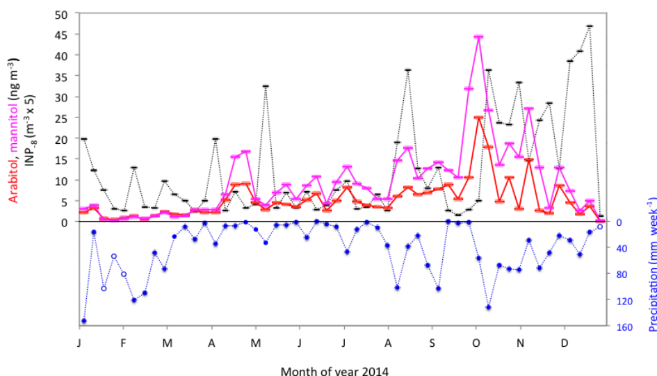
Figure 5. Weekly concentration of arabitol (red) and mannitol (magenta). The time courses of INP 8 in PM 10 (black; \times 5 , to fit onto the same scale) and precipitation (blue) are copied from Fig. 1 to facilitate direct comparison.
