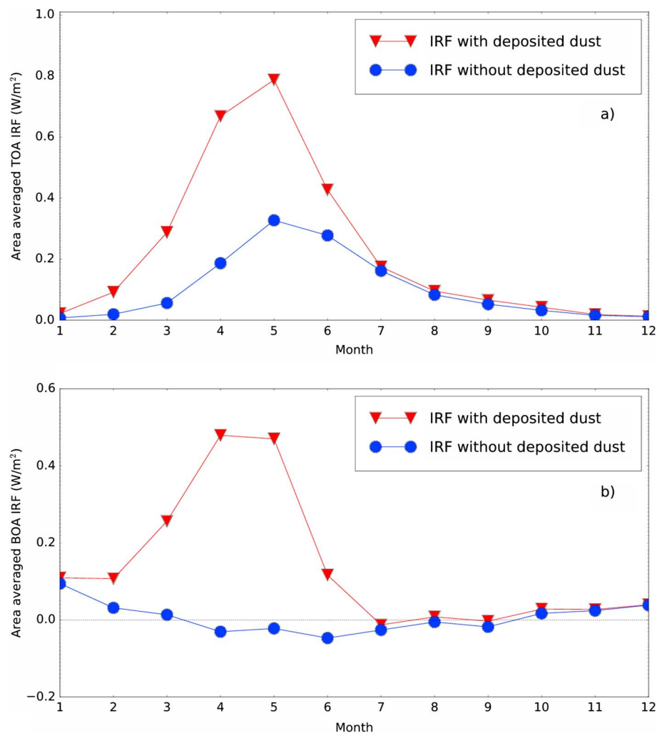
Figure 1. The area averaged (north of 60°N) dust (a) top of the atmosphere (TOA) and (b) bottom of the atmosphere (BOA) instantaneous radiative forcing (IRF) for 2012 conditions. The red (blue) curves show the IRF including (excluding) dust deposited on the surface. The black dotted line in panel (b) indicates the zero line.
