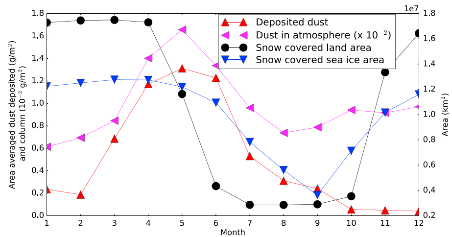
Figure 2. Annual variation of the land area covered by snow, the sea ice area covered by snow, the area-averaged monthly deposited dust (on snow covered areas), and the atmospheric dust column in the year 2012.
