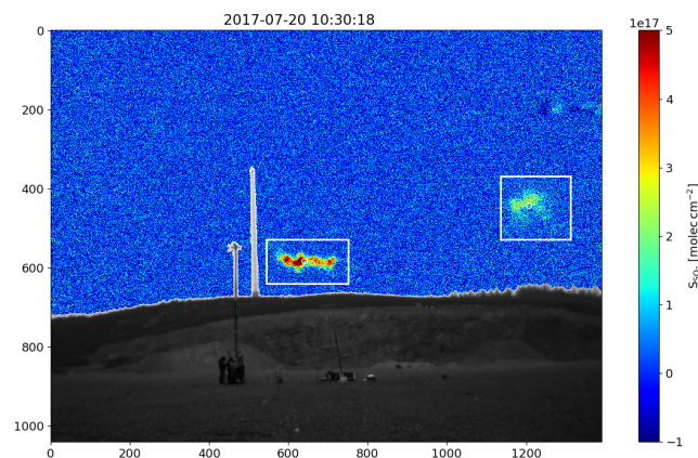
Figure 6. Example of a SO 2 CIC image from a SO 2 camera (camera 4). The image contains two SO 2 puffs marked by the detected ROI (white rectangle). Artefacts produced by a cloud are visible in the upper right corner.
