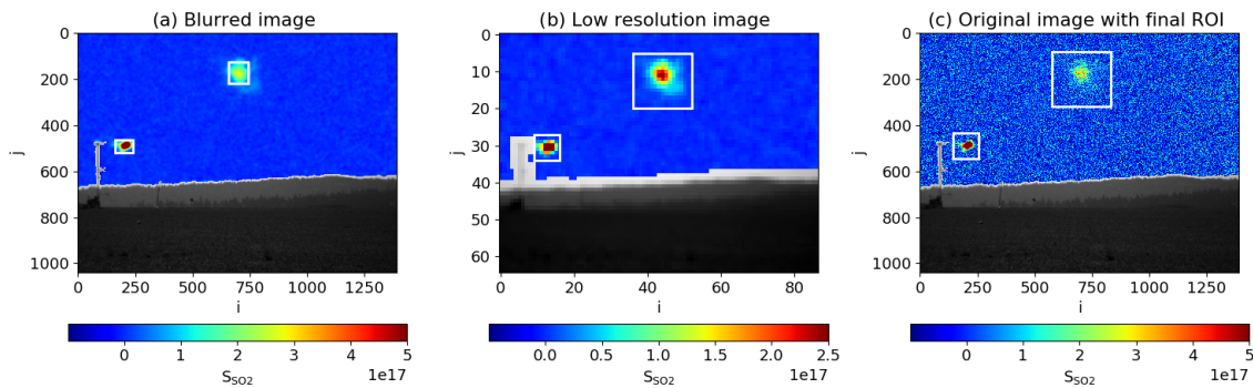
Figure B2. Puff detection based on noise-reduced images, here for camera 1 at 10:30:12. The ROI is detected in a blurred image based on the position of the CM in the previous image (a). A low resolution image is used to detect connected areas above a threshold (b). The combination of both detections gives the resulting ROI, which is used to calculate the CM, total signal and spread in the original image (c).
