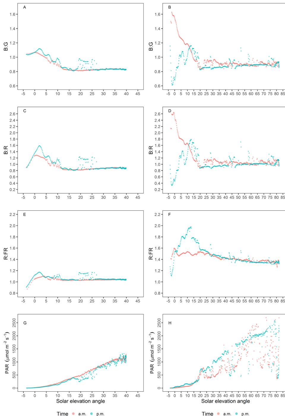
Fig. 4. A-H. Spectral photon ratios and PAR irradiance calculated from spectral irradiance measurements from Gual Pahari, India, plotted against solar elevation angle. The left-hand panels (A, C, E and G) present measurements from 11.1.2017, a relatively sunny and cloud-free day with water vapour column average 0.61 cm (min 0.50 cm, max 0.83 cm) and total ozone 260 DU. The right-hand panels (B, D, F, H) are 21.7.2017, a variably cloudy day with water vapour column average 5.9 cm (min 5.3 cm, max 6.9 cm) and total ozone 276 DU. Clouds obscuring the sun make a dip in the PAR irradiance graphs (G and H). Red circles are measurements before noon and blue circles after noon, recorded once per minute. Please note that the scales on the x-axis and y-axis are different from those in Fig. 3.
